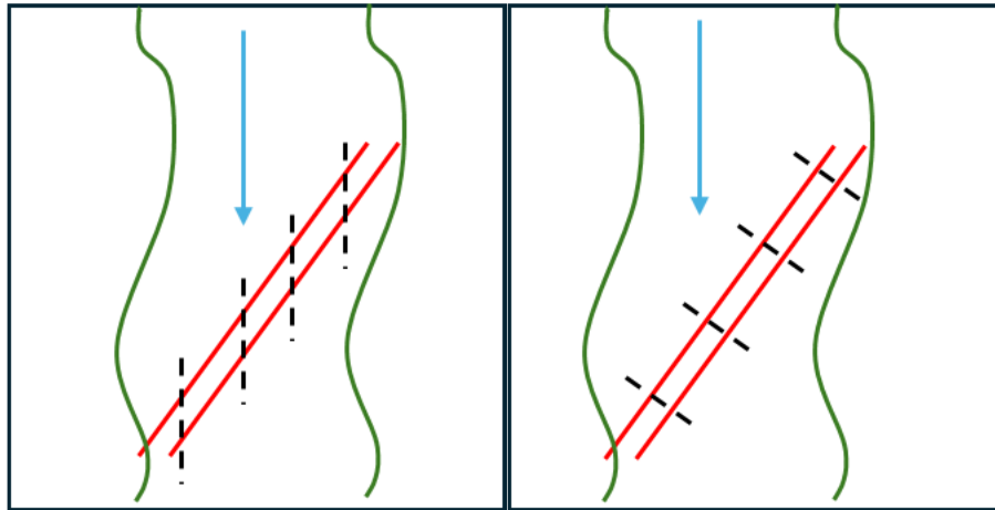
Figure 12: Sketch indicating orientation of correct orientation of culverts (black dashed lines) relative to the flow of water (blue arrow) and the alignment of the road (red lines).
