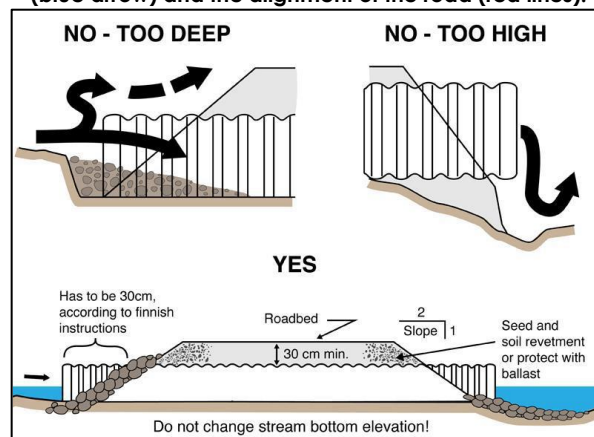
Figure 13: Diagram illustrating the ideal placement of culverts relative to the bed of the wetland.
