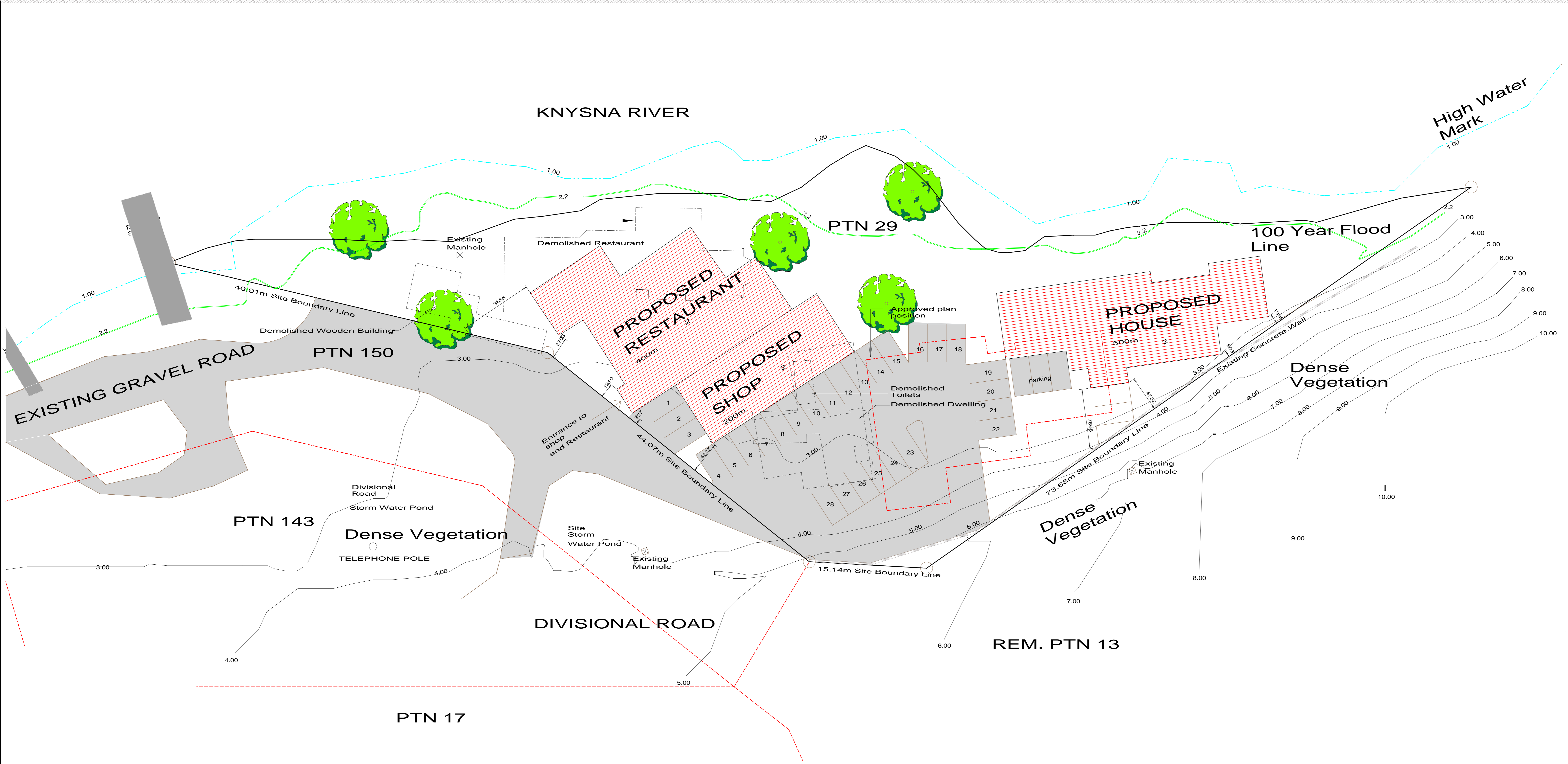
Site development plan 1:200
