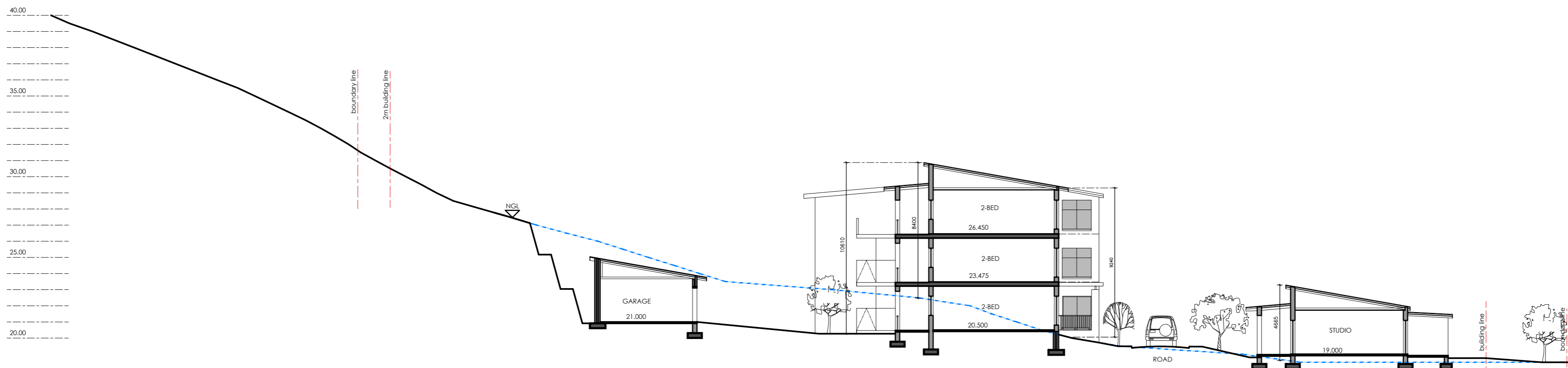
SECTION B-B: 2-BED UNITS & STUDIOS
